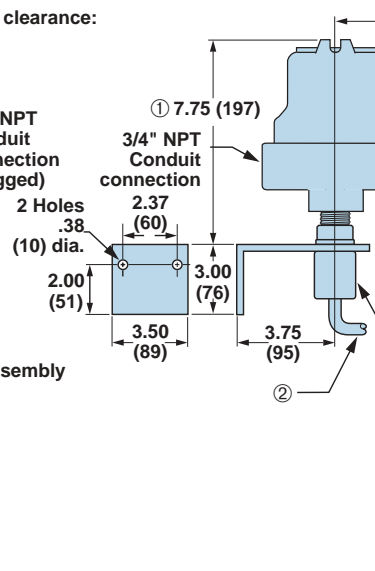
Remote Mount with Standard Rigid Probe
