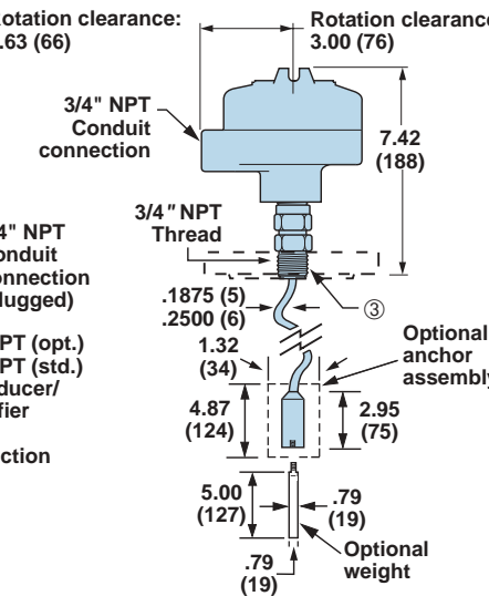
Remote Mount with Flexible Probe
