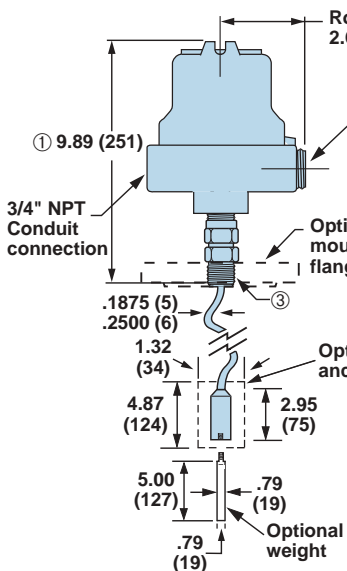
Integral Mount with Flexible Probe
