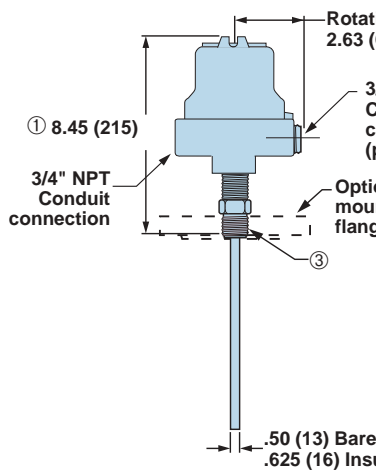
Integral Mount with Standard Rigid Probe
