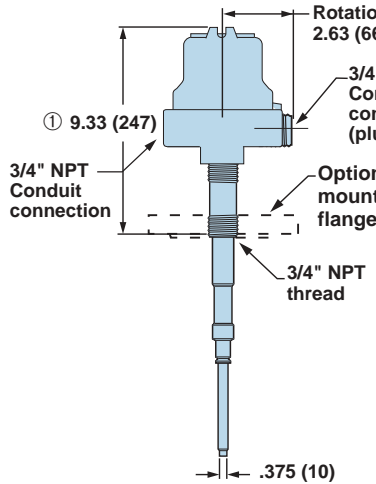
Integral Mount with Guarded Probe
