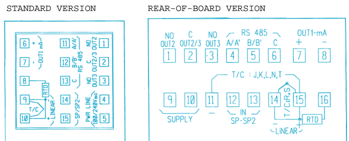
REAR TERMINAL BLOCK LFS mA
