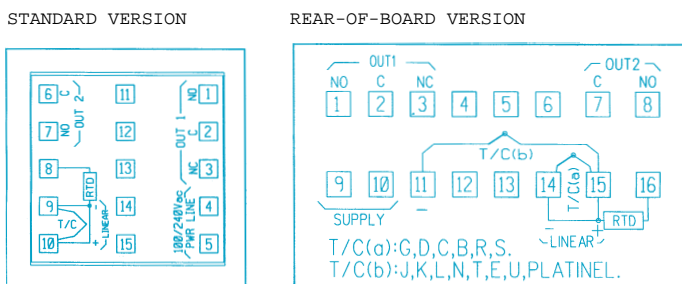
Figure 10 REAR TERMINAL BLOCK without RS-485
