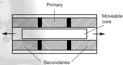
Fig A) LVDT cross sectional diagram
